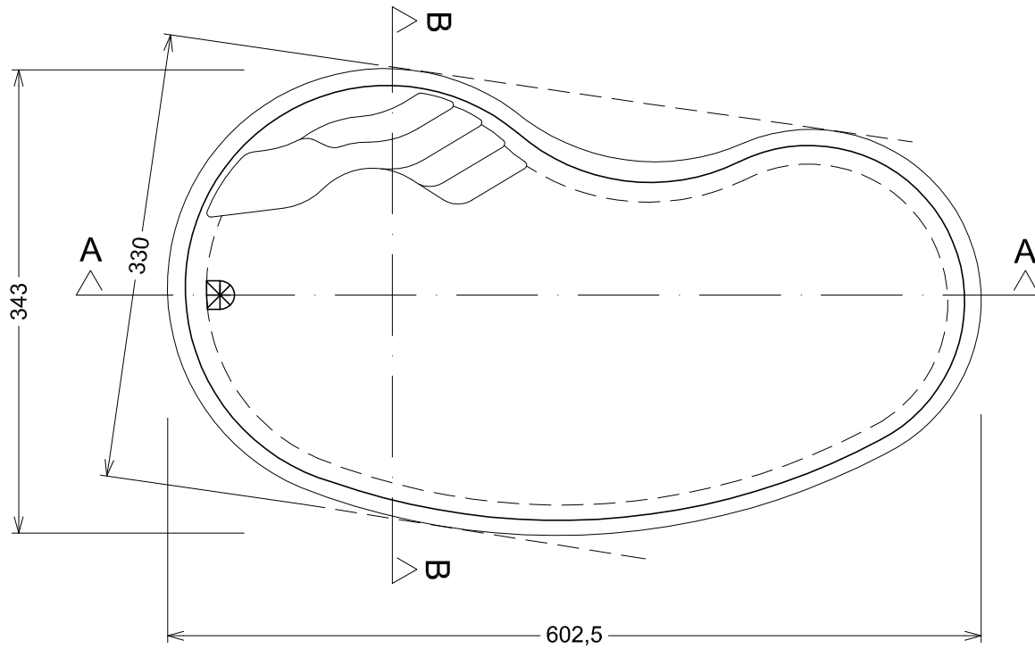
Grundriss - Ground plan
